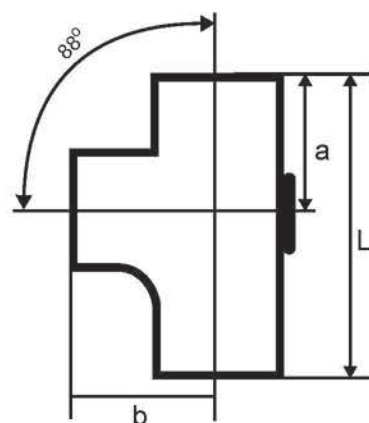
88° Single Branch with Access Door 多口三叉
