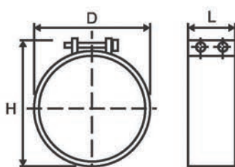
Type 'CH' Stainless Steel Coupling (SS 304 / SS316) 不銹鋼喉箍
