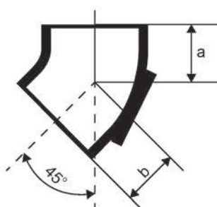
45° Bend with Access Door 多口短邊
